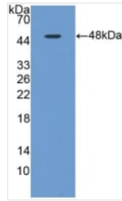
WB (Western Blot) Western Blot: Sample: Recombinant MAPt, Rat.
