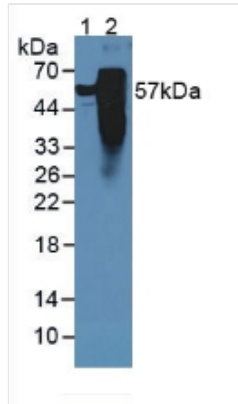
WB (Western Blot) Western Blot: Sample: Lane1: Rat Serum; Lane2: Rat Brain Tissue.
