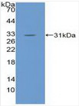
WB (Western Blot) Western Blot: Sample: Recombinant EGFL7, Mouse.
