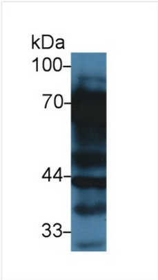
WB (Western Blot) Western Blot: Sample: Rat Liver lysate; Primary Ab: 3ug/ml Rabbit Anti-Rat VTN Antibody Second Ab: 0.2ug/mL HRP-Linked Caprine Anti-Rabbit IgG Polyclonal Antibody
