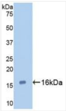
WB (Western Blot) Western Blot: Sample: Recombinant GAL7, Human.
