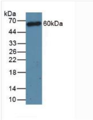
WB (Western Blot) Western Blot: Sample: Mouse Thymus Tissue.
