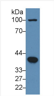
WB (Western Blot) Western Blot: Sample: Human Hela cell lysate; Primary Ab: 3ug/ml Rabbit Anti-Human BMP2 Antibody Second Ab: 0.2ug/mL HRP-Linked Caprine Anti-Rabbit IgG Polyclonal Antibody
