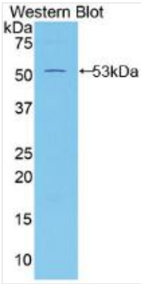
WB (Western Blot) Figure. Western Blot; Sample: Recombinant MSLN, Mouse.
