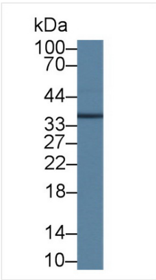
WB (Western Blot) Western Blot: Sample: Rat Lymph node lysate; Primary Ab: 2ug/ml Rabbit Anti-Human UCP2 Antibody Second Ab: 0.2ug/mL HRP-Linked Caprine Anti-Rabbit IgG Polyclonal Antibody
