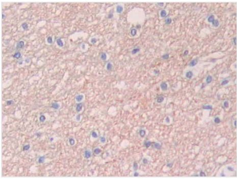
IHC (Immunohistochemisry) DAB staining on formalin fixed paraffin- embedded kidney tissue
