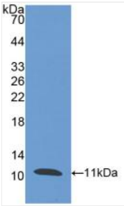
WB (Western Blot) Western Blot: Sample: Recombinant PI3, Human.
