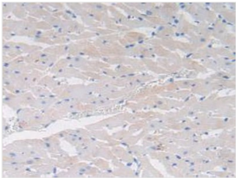
IHC (Immunohistochemisry) DAB staining on IHC-P; Samples: Rat Heart Tissue.
