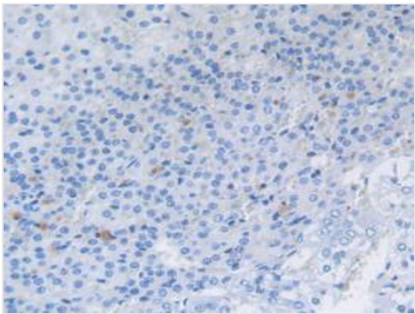
IHC (Immunohiostchemistry) DAB staining on IHC-P; Samples: Rat Adrenal Gland Tissue.
