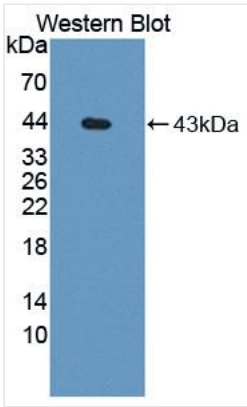
WB (Western Blot) Western Blot: Sample: Recombinant CCK, Rat.
