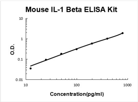
Standard Curve (Sample) Mouse IL-1 beta PicoKine ELISA Kit standard curve
