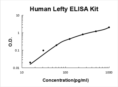
Standard Curve (Sample) Human Lefty PicoKine ELISA Kit standard curve
