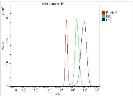
FCM/FACS (Flow Cytometry) Figure 2. Flow Cytometry analysis of HepG2 cells using anti-Lysozyme/LYZ antibody (AAA127082).Overlay histogram showing HepG2 cells stained with AAA127082 (Blue line). The cells were fixed with 4% paraformaldehyde and blocked with 10% normal goat serum. And then incubated with rabbit anti-Lysozyme/LYZ Antibody (AAA127082, 1ug/1x10 6 cells) for 30 min at 20 degree C. DyLight488 conjugated goat anti-rabbit IgG was used as secondary antibody for 30 minutes at 20 degree C. Isotype control antibody (Green line) was rabbit IgG (1ug/1x10 6 ) used under the same conditions. Unlabelled sample (Red line) was also used as a control.
