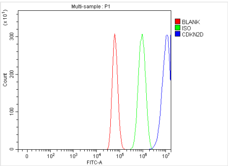
FCM/FACS (Flow Cytometry) Figure 2. Flow Cytometry analysis of U87 cells using anti-P19 INK4d/CDKN2D antibody (AAA126380).Overlay histogram showing U87 cells stained with AAA126380 (Blue line). The cells were blocked with 10% normal goat serum. And then incubated with rabbit anti-P19 INK4d/CDKN2D Antibody (AAA126380, 1 ug/1x10 6 cells) for 30 min at 20 degree C. DyLight488 conjugated goat anti-rabbit IgG was used as secondary antibody for 30 minutes at 20 degree C. Isotype control antibody (Green line) was rabbit IgG (1 ug/1x10 6 ) used under the same conditions. Unlabelled sample (Red line) was also used as a control.
