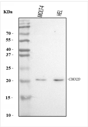
WB (Western Blot) Figure 1. Western blot analysis of P19 INK4d/CDKN2D using anti-P19 INK4d/CDKN2D antibody (AAA126380).Electrophoresis was performed on a 5-20% SDS-PAGE gel at 70V (Stacking gel)/90V (Resolving gel) for 2-3 hours. The sample well of each lane was loaded with 30 ug of sample under reducing conditions.Lane 1: human MOLT4 whole cell lysates,Lane 2: human HEL whole cell lysates.After electrophoresis, proteins were transferred to a nitrocellulose membrane at 150 mA for 50-90 minutes. Blocked the membrane with 5% non-fat milk/TBS for 1.5 hour at RT. The membrane was incubated with rabbit anti-P19 INK4d/CDKN2D antigen affinity purified polyclonal antibody (#AAA126380) at 0.5 ug/mL overnight at 4 degree C, then washed with TBS-0.1%Tween 3 times with 5 minutes each and probed with a goat anti-rabbit IgG-HRP secondary antibody at a dilution of 1:5000 for 1.5 hour at RT. The signal is developed using an Enhanced Chemiluminescent detection (ECL) kit with Tanon 5200 system. A specific band was detected for P19 INK4d/CDKN2D at approximately 18 kDa. The expected band size for P19 INK4d/CDKN2D is at 18 kDa.
