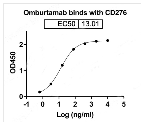
Bioactivity Detects Human CD276 in direct ELISAs.
