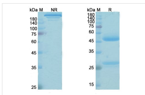
SDS-PAGE SDS PAGE for Omburtamab
