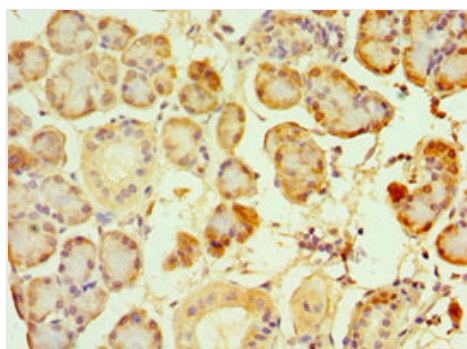
IHC (Immunohistochemistry) Immunohistochemistry of paraffin-embedded human pancreas using AAA118384 at dilution 1:100
