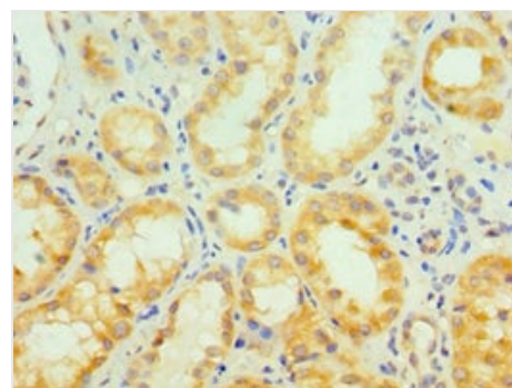
IHC (Immunohistochemistry) Immunohistochemistry of paraffin-embedded human kidney using AAA118384 at dilution 1:100
