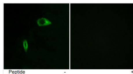
IF (Immunofluorescence)
