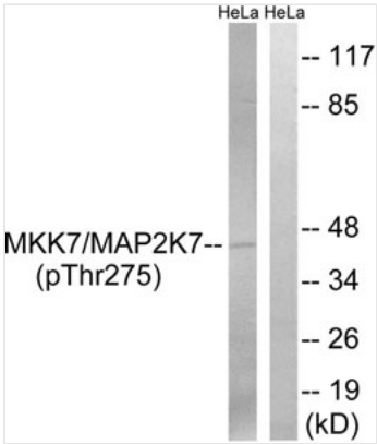
WB (Western Blot) Western blot analysis of extracts from HeLa cells, treated with calyculinA (50ng/ml, 30mins), using MAP2K7 (Phospho-Thr275) antibody.
