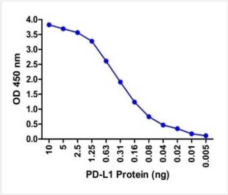
ELISA A sandwich ELISA was performed using the anti-PD-L1 mAb (5 µg/ml) as the capture antibody. Biotin-labeled anti-PD-L1 mAb (1 µg/ml) and streptavidin-HRP (0.1 µg/ml) were used for detection. Detection range is from 10 ng to 20 pg.
