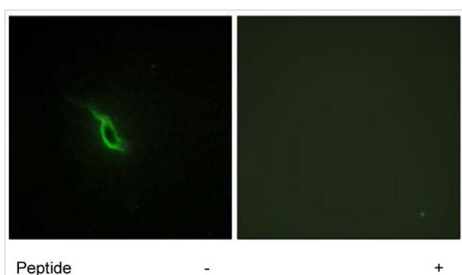
IF (Immunofluorescence)
