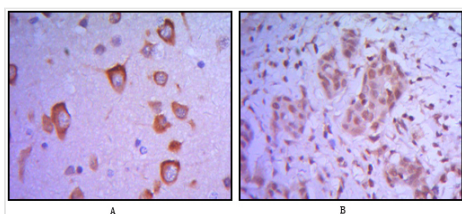
IHC (Immunohistochemistry)
