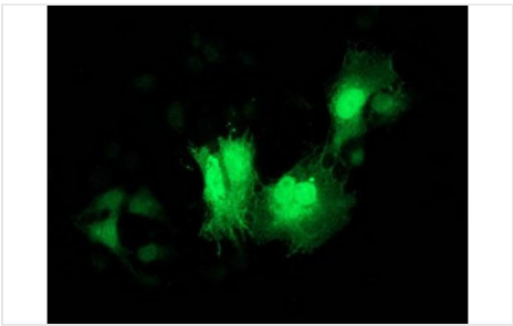
IF (Immunofluorescence) Immunofluorescent staining of COS7 cells transiently transfected with recombinant CDK2 protein using CDK2 antibody
