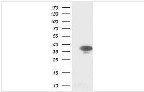
WB (Western Blot) Western Blot analysis of HEK293T cell lysates (5 ug) transfected with either recombinant CDK2 protein (Right) or empty vector (Left) detected with CDK2 antibody
